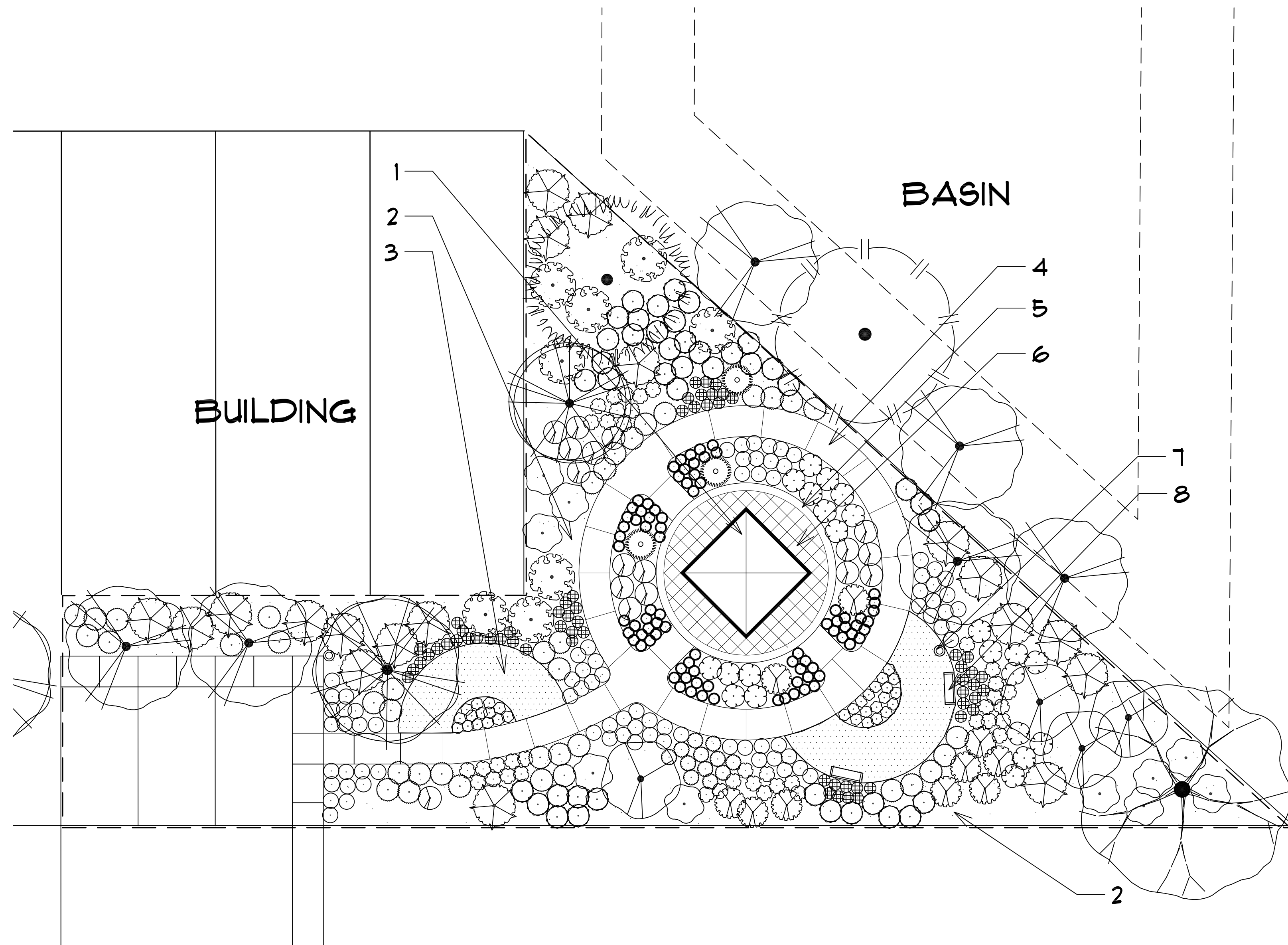
A: POLLINATOR GARDEN PLAN
