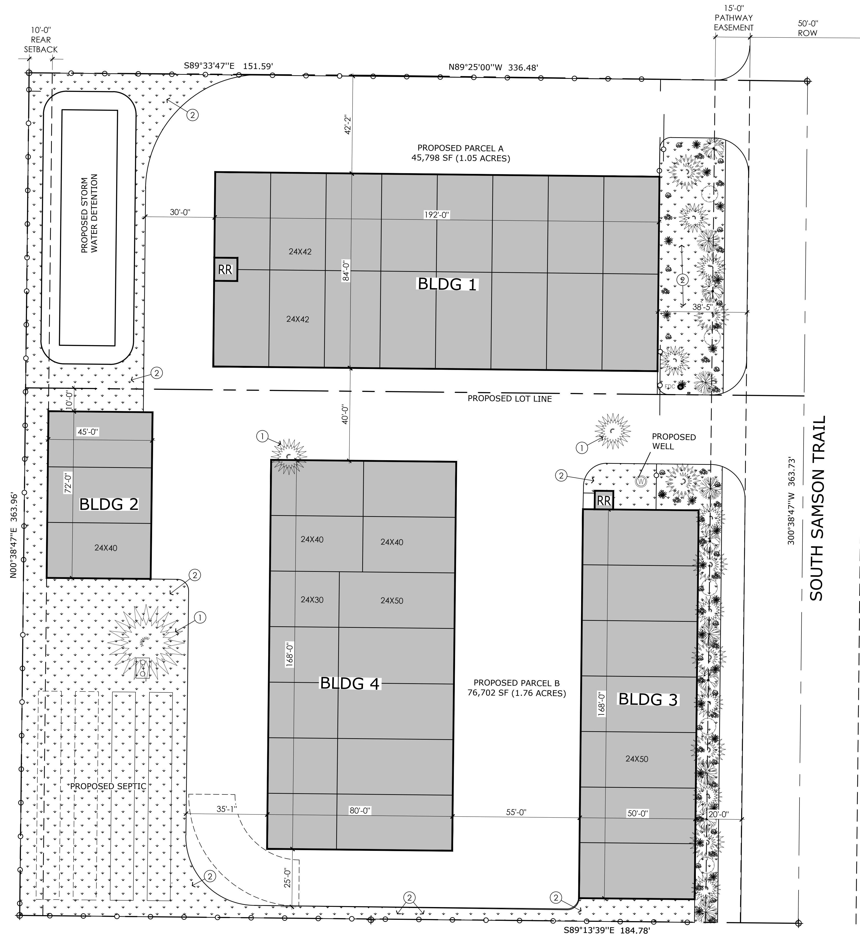
SITE LANDSCAPE PLAN SCALE: 1"=20'-0"
